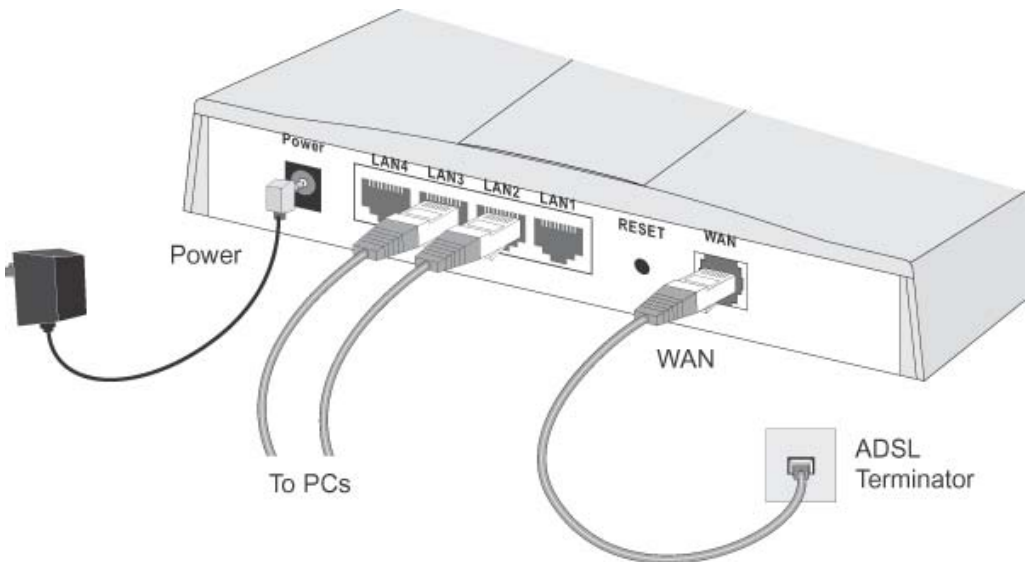
Figure 4: Installation Diagram
